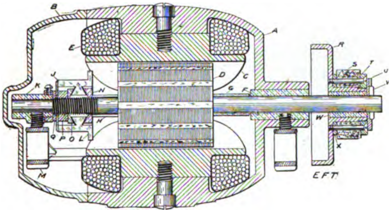
FIG. 343. —Sectional Diagram of the Apple Igniting Dynamo. The parts shown are: A, cast iron body containing the moving parts; B, the hinged lid of the body; C, the one-pole piece of the field magnets; D, the armature; E, the coil of one of the field magnets; F, brass bearing of the armature spindle; G and H, fibre tubes surrounding the spindle; K, brass spider supporting the spindle; L, commutator; M, wick feed oil cup; N, beveled nut supporting the commutator; O, P, Q, supports of the commutator; R, the driving disc; S, lever friction pinion.
